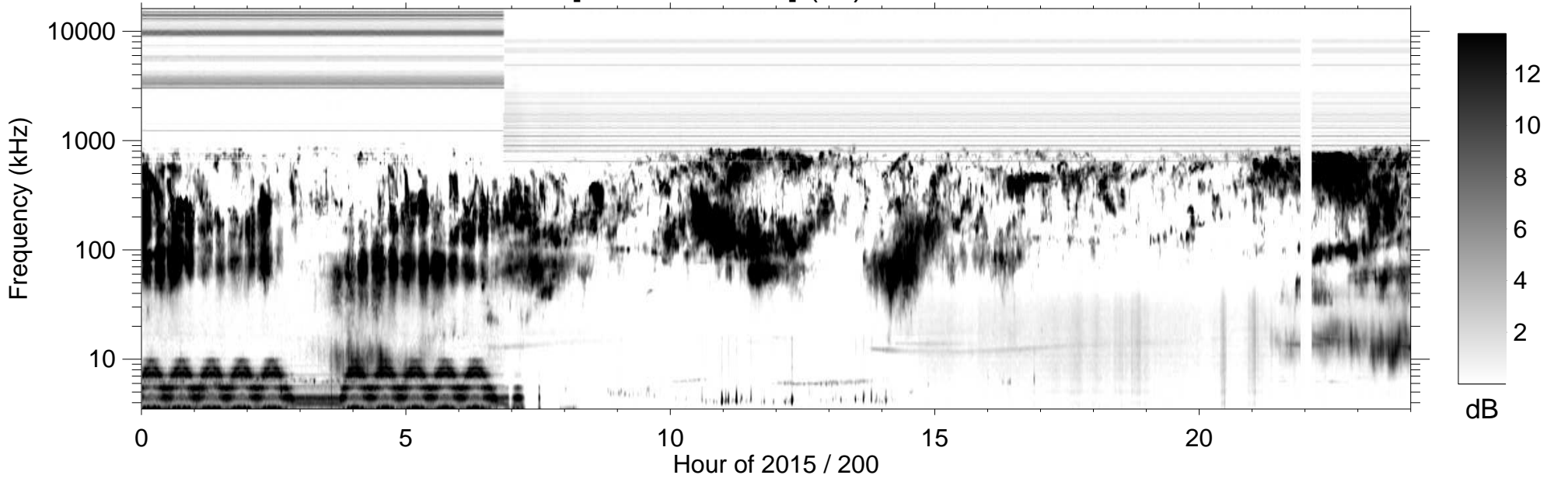
RPWS [ABCH1H2/Ex] (-B) 2015/07/19
