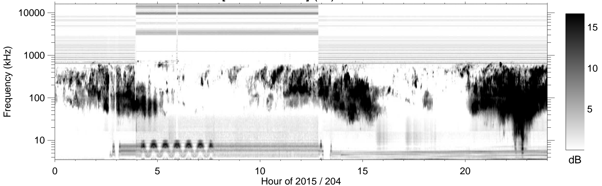
RPWS [ABCH1H2/Ex] (-B) 2015/07/23
