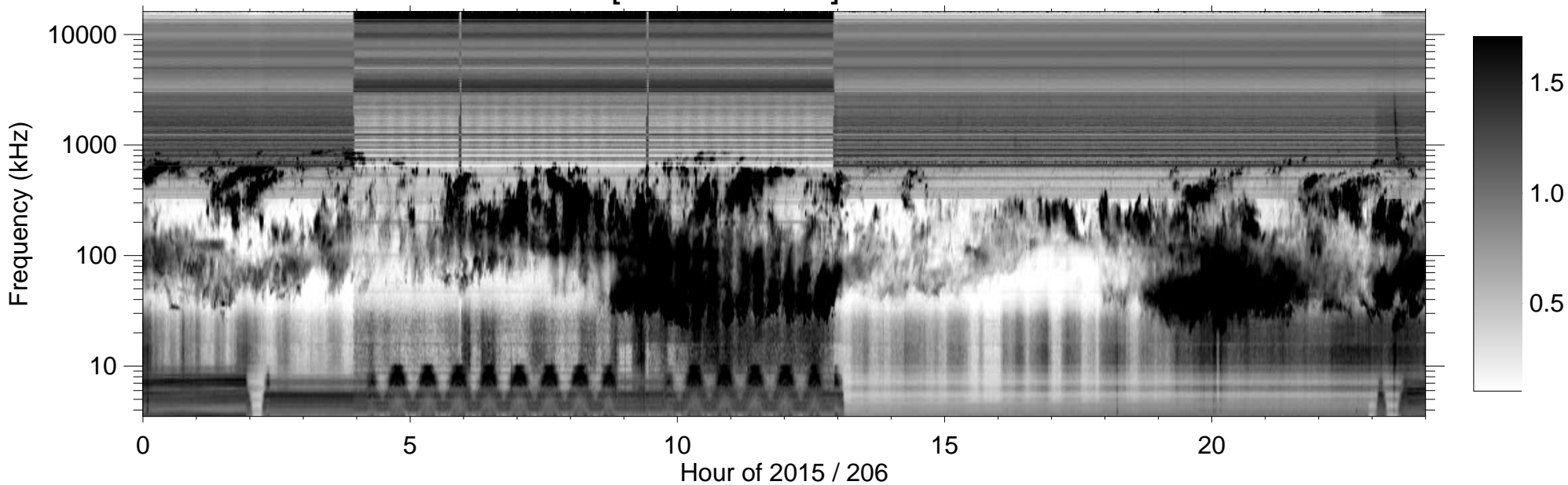
RPWS [ABCH1H2/Ex] (-B) 2015/07/25
