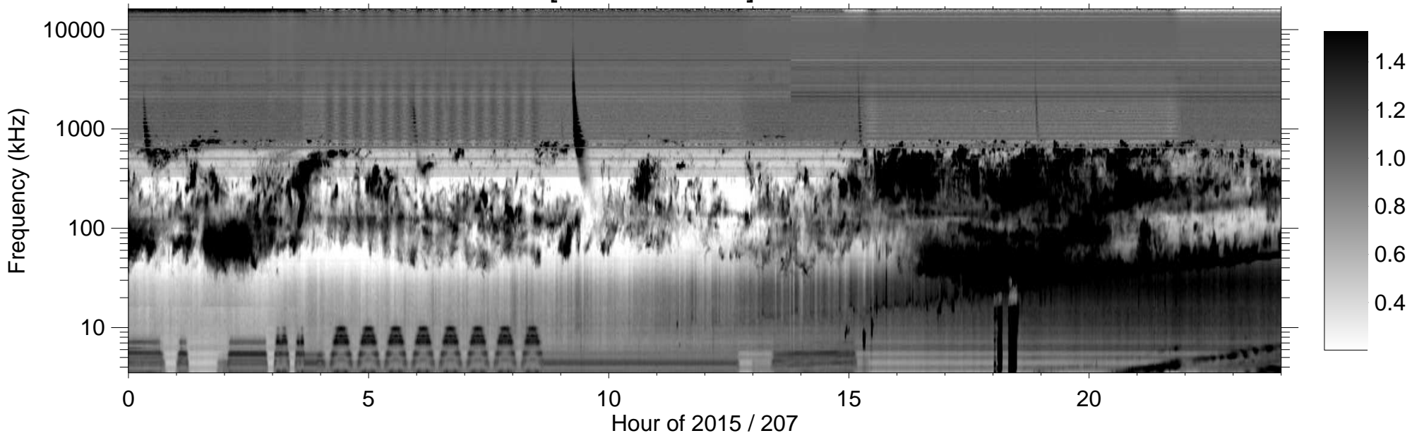
RPWS [ABCH1H2/Ex] (-B) 2015/07/26
