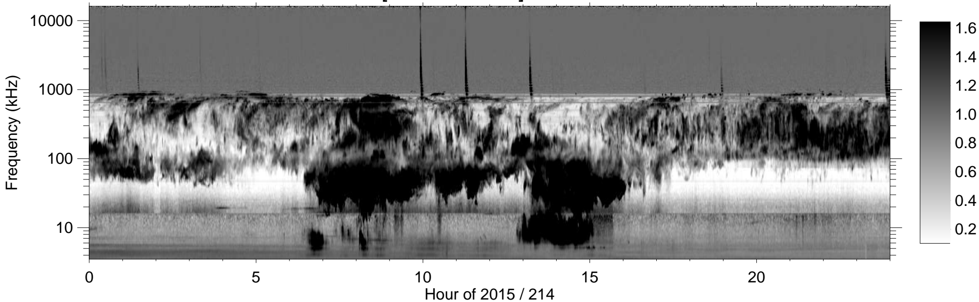
RPWS [ABCH1H2/Ex] (-B) 2015/08/02
