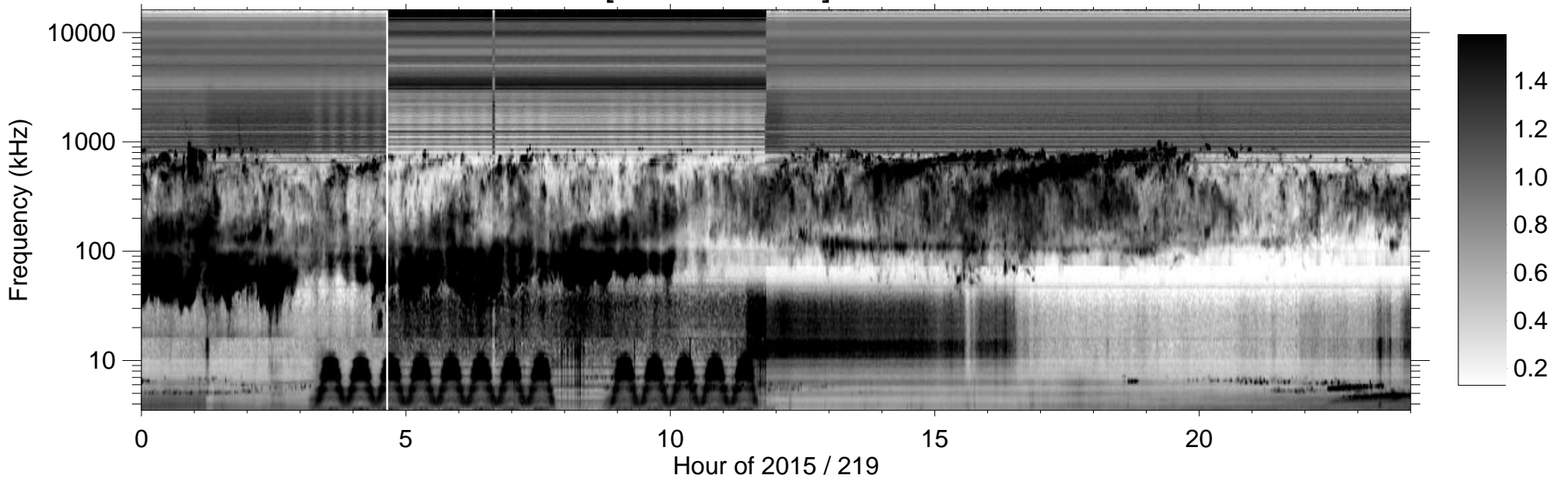
RPWS [ABCH1H2/Ex] (-B) 2015/08/07
