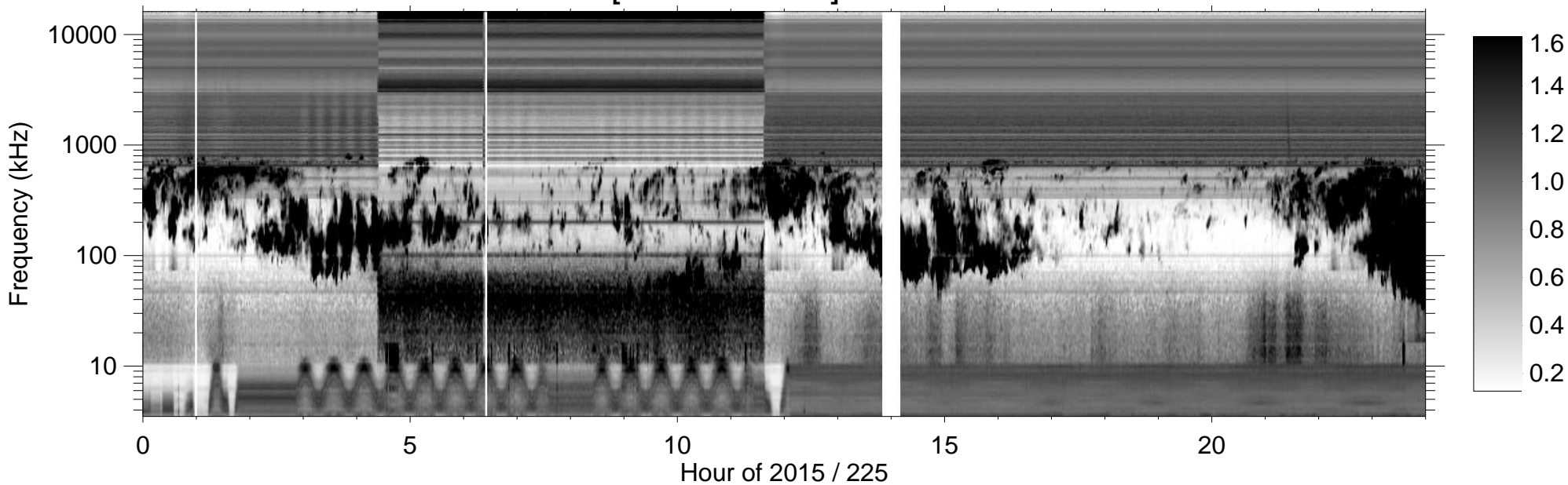
RPWS [ABCH1H2/Ex] (-B) 2015/08/13
