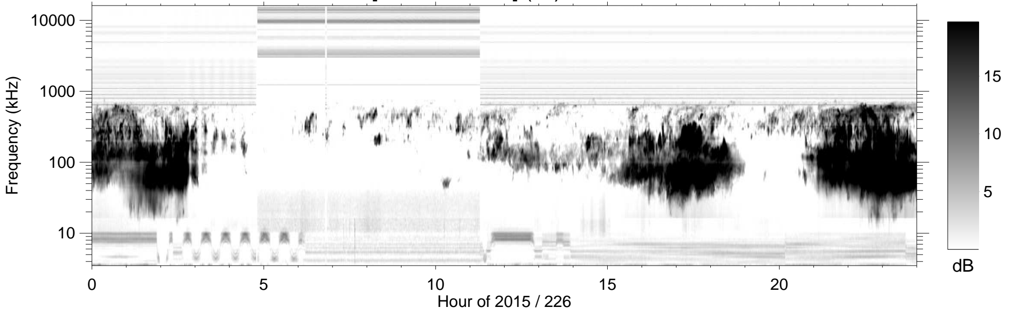
RPWS [ABCH1H2/Ex] (-B) 2015/08/14
