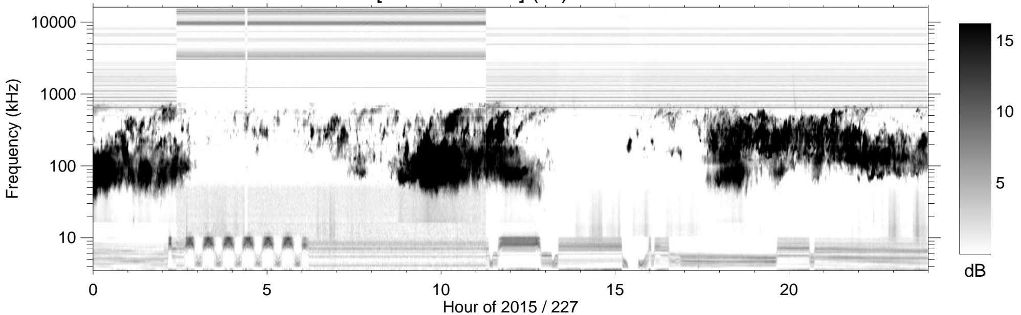
RPWS [ABCH1H2/Ex] (-B) 2015/08/15
