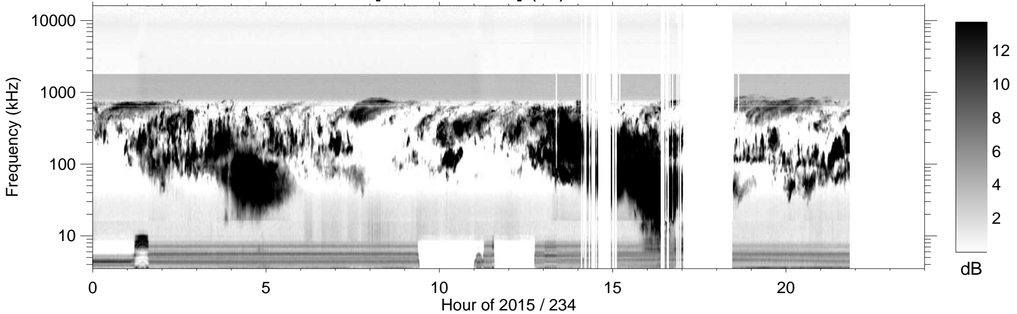
RPWS [ABCH1H2/Ex] (-B) 2015/08/22
