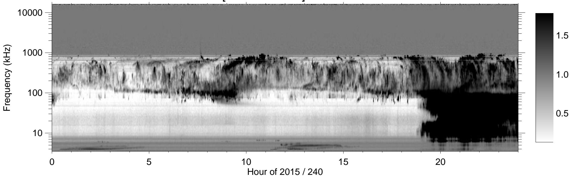
RPWS [ABCH1H2/Ex] (-B) 2015/08/28
