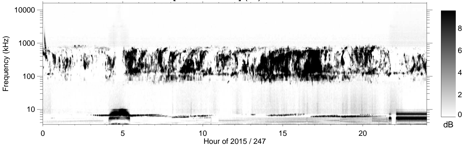
RPWS [ABCH1H2/Ex] (-B) 2015/09/04
