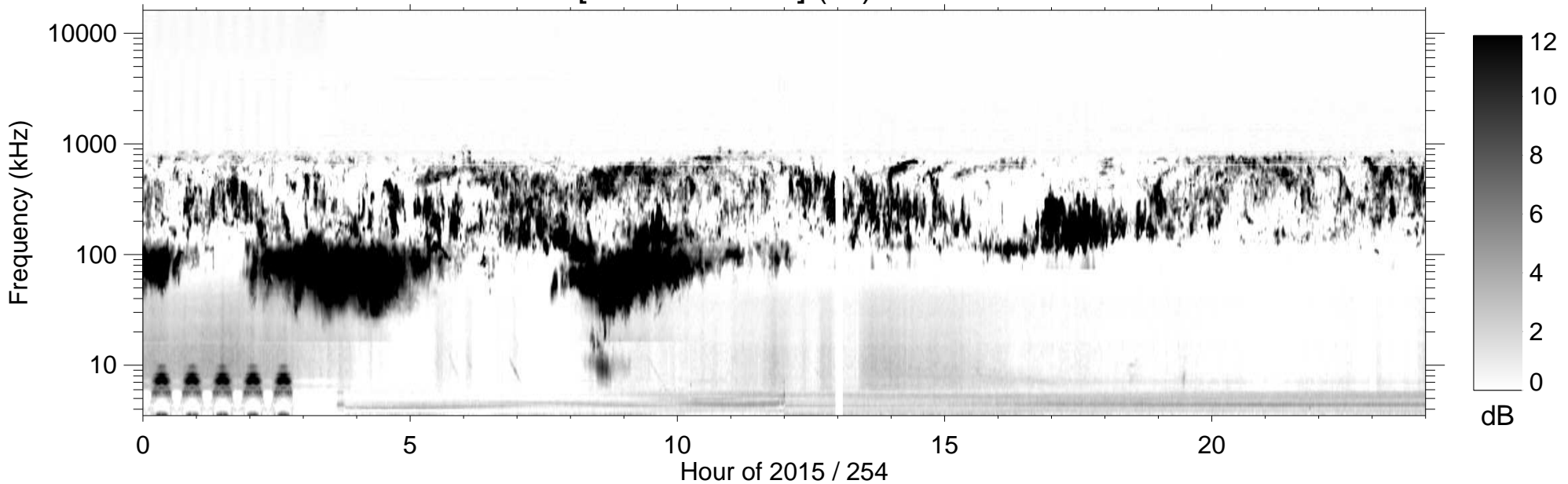
RPWS [ABCH1H2/Ex] (-B) 2015/09/11
