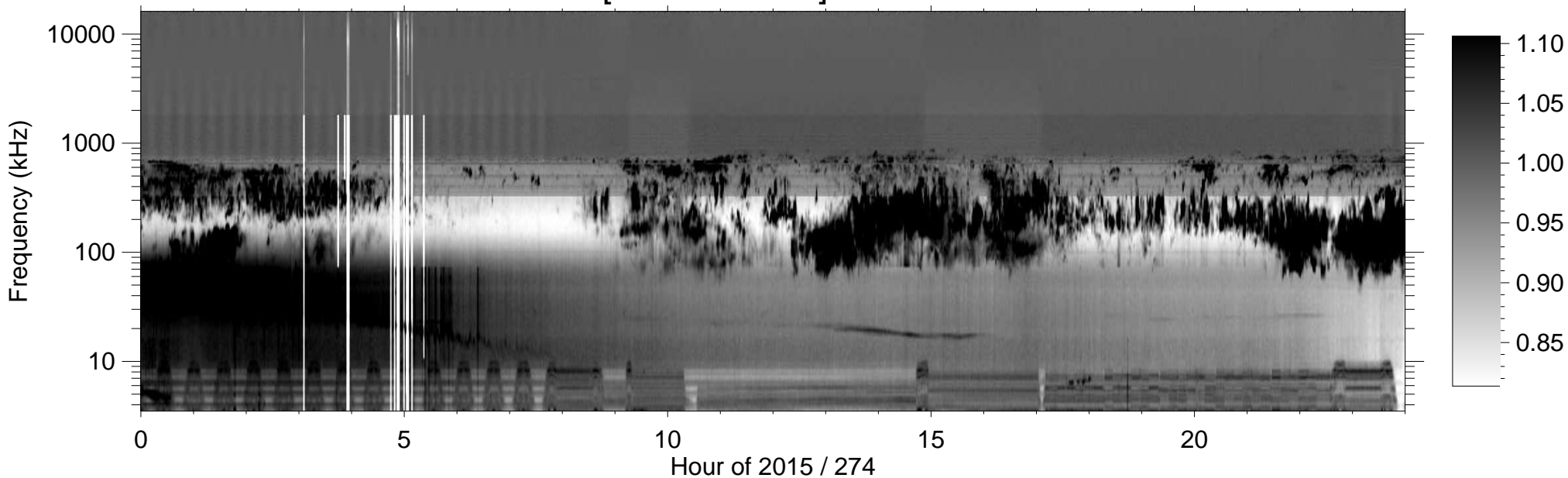
RPWS [ABCH1H2/Ex] (-B) 2015/10/01
