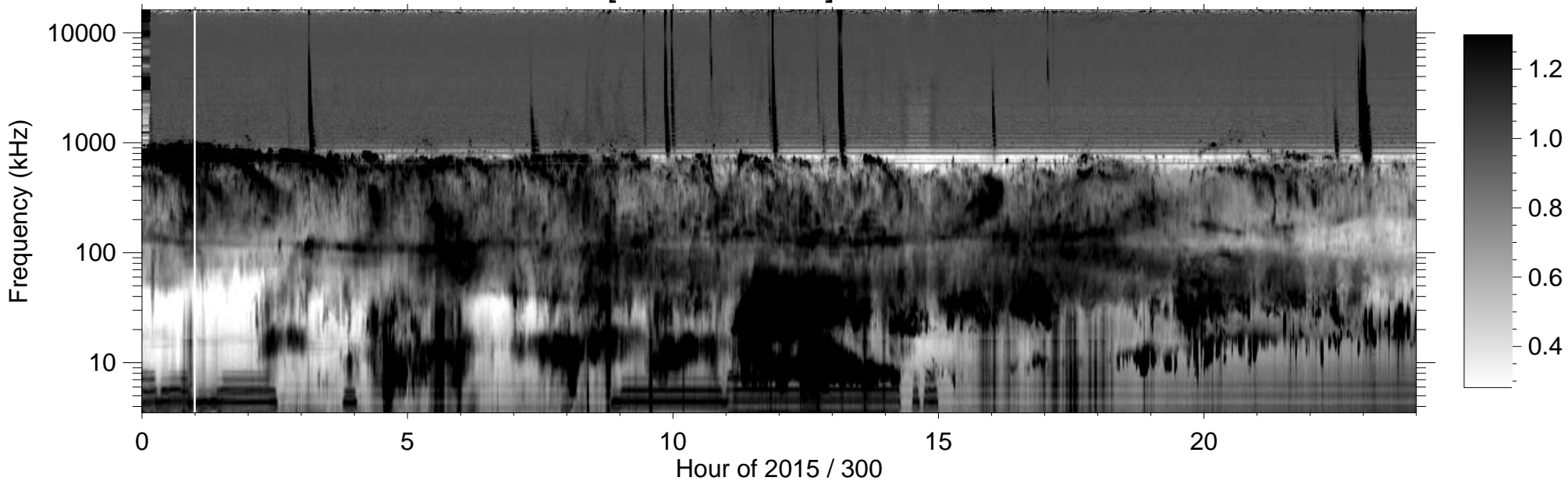
RPWS [ABCH1H2/Ex] (-B) 2015/10/27
