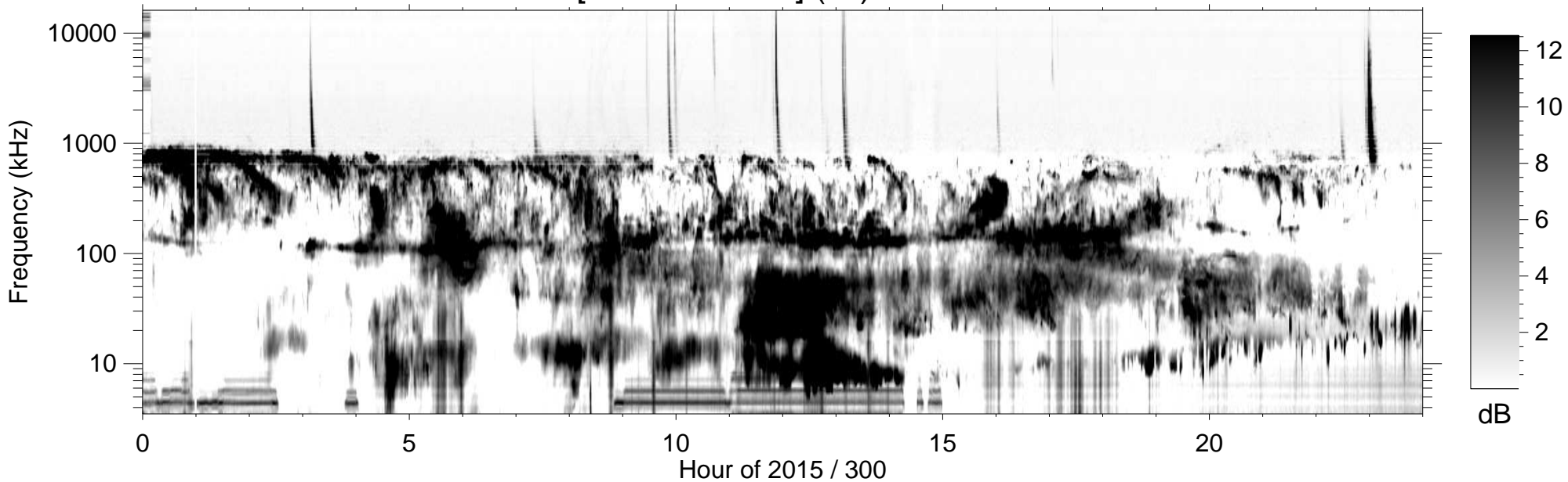
RPWS [ABCH1H2/Ex] (-B) 2015/10/27
