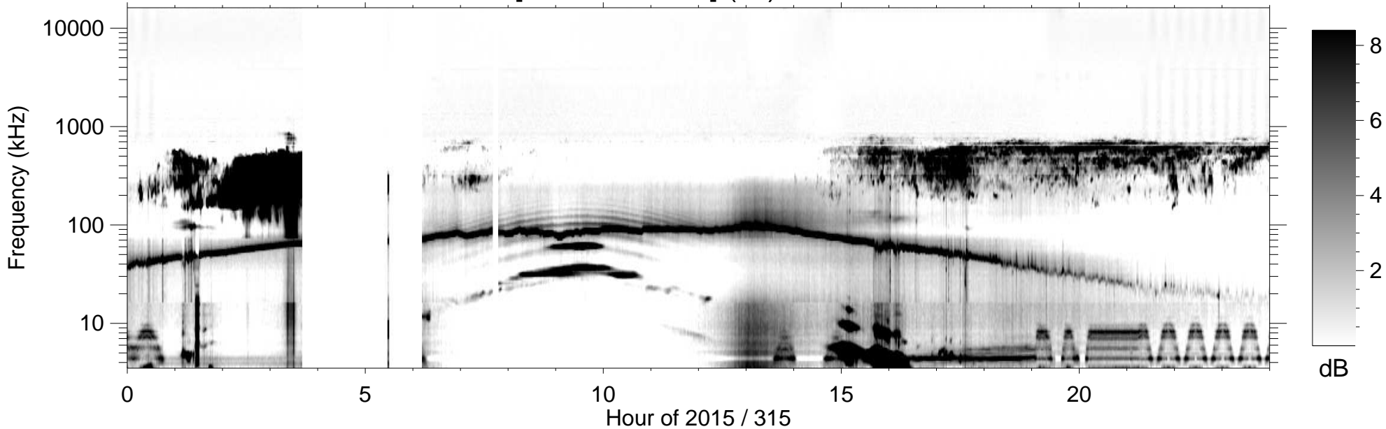
RPWS [ABCH1H2/Ex] (-B) 2015/11/11
