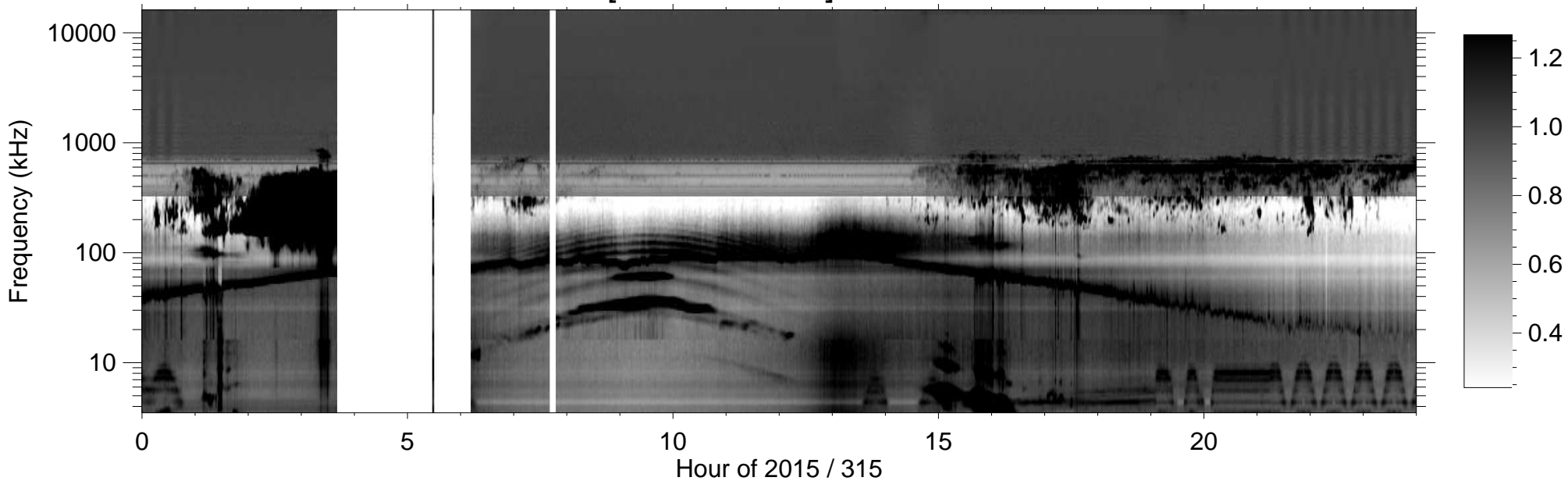
RPWS [ABCH1H2/Ex] (-B) 2015/11/11
