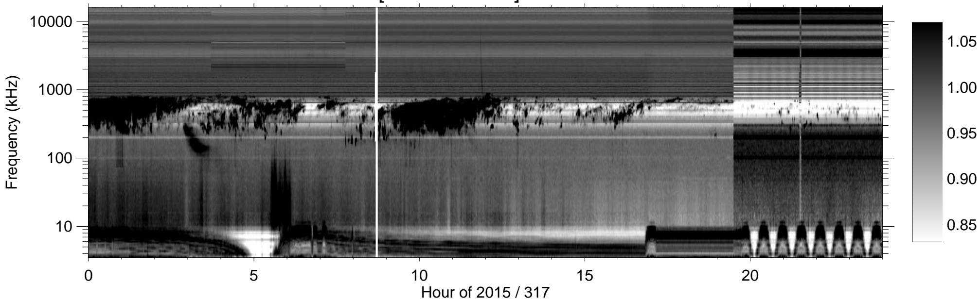
RPWS [ABCH1H2/Ex] (-B) 2015/11/13
