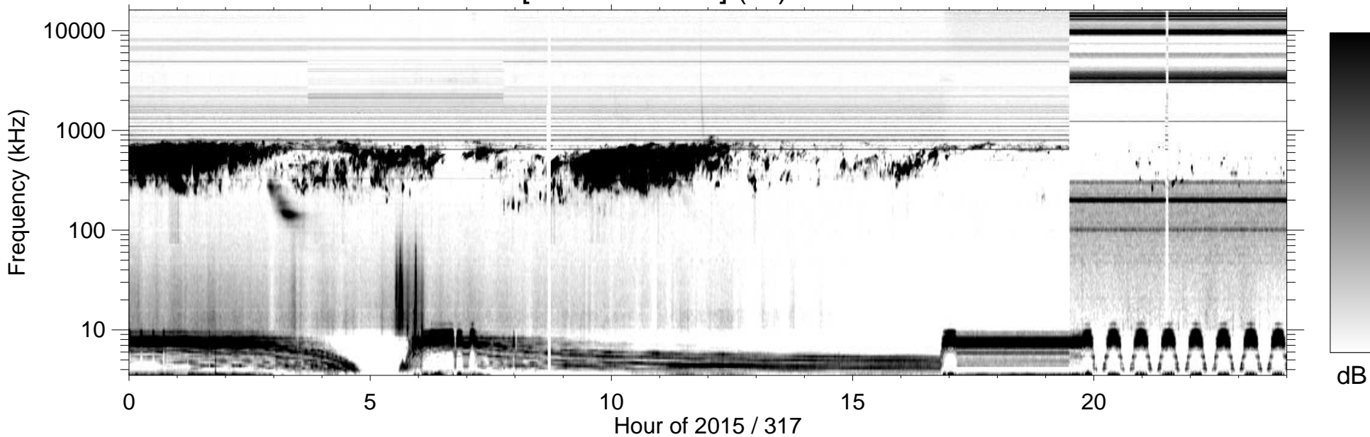
RPWS [ABCH1H2/Ex] (-B) 2015/11/13
