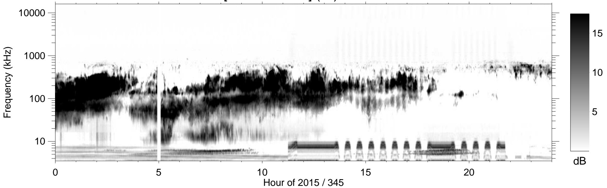
RPWS [ABCH1H2/Ex] (-B) 2015/12/11
