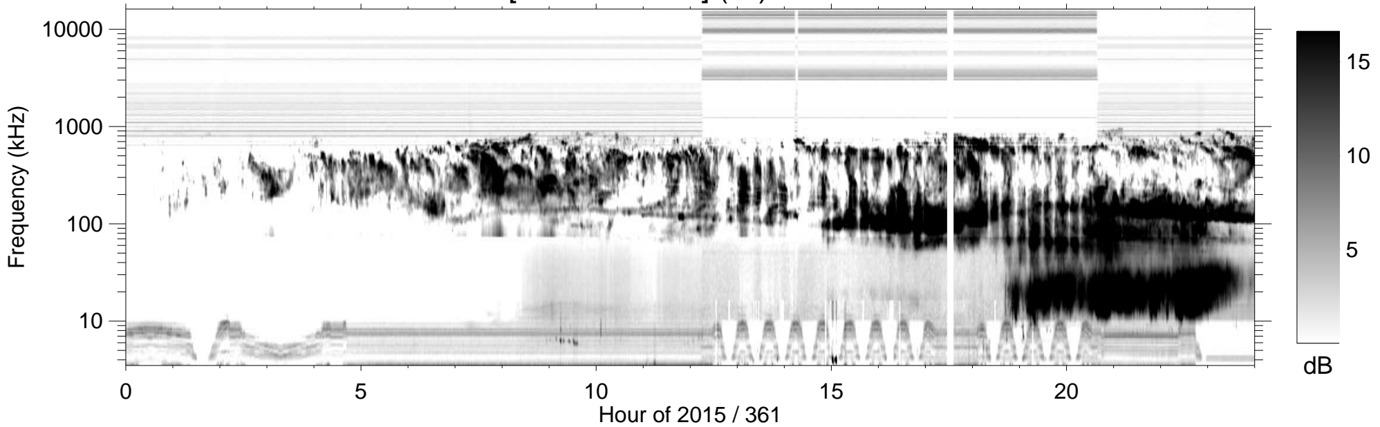
RPWS [ABCH1H2/Ex] (-B) 2015/12/27
