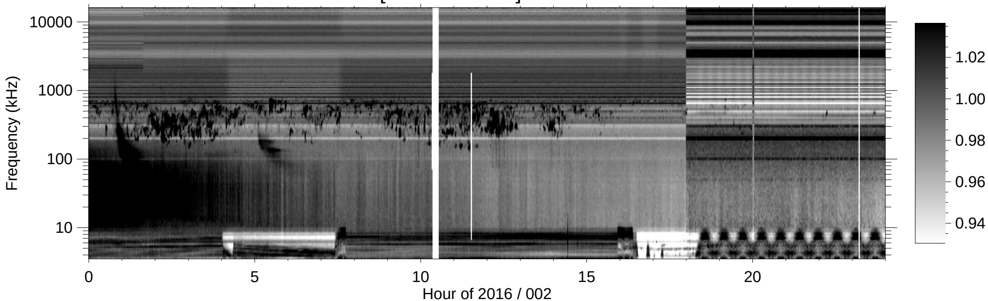
RPWS [ABCH1H2/Ex] (-B) 2016/01/02
