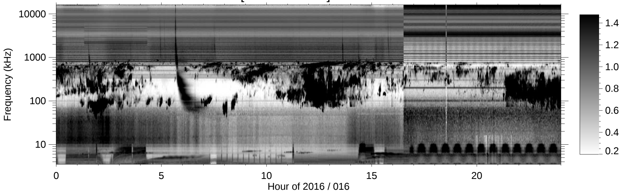
RPWS [ABCH1H2/Ex] (-B) 2016/01/16
