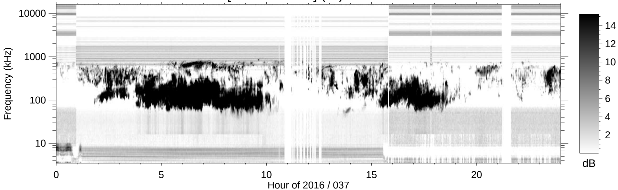
RPWS [ABCH1H2/Ex] (-B) 2016/02/06
