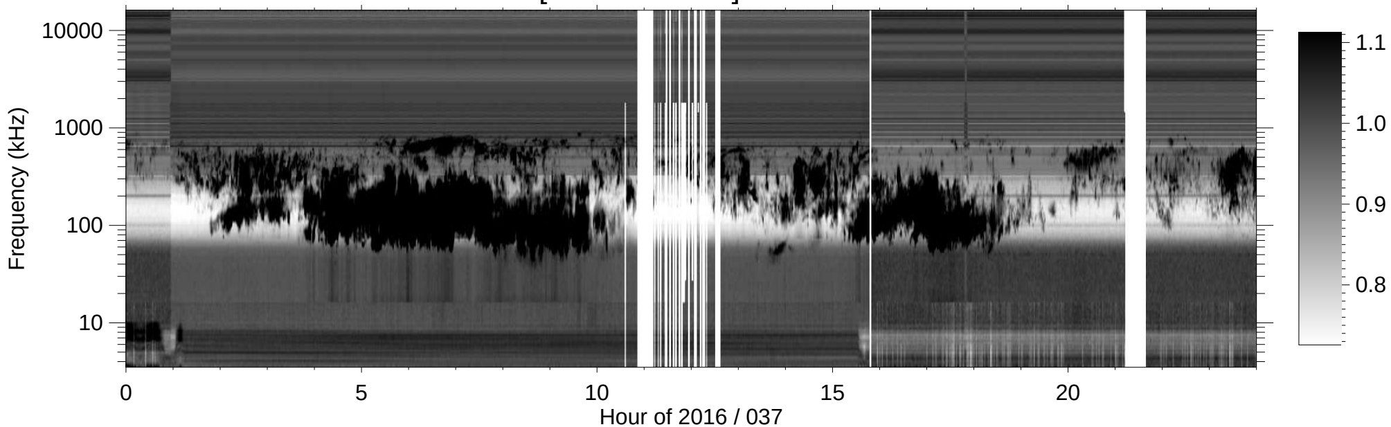
RPWS [ABCH1H2/Ex] (-B) 2016/02/06
