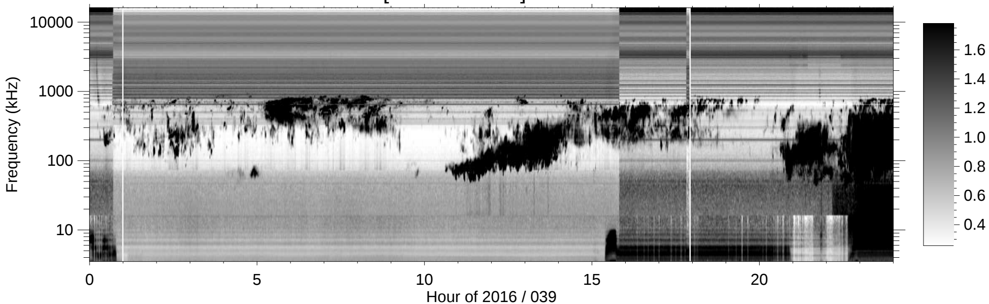
RPWS [ABCH1H2/Ex] (-B) 2016/02/08
