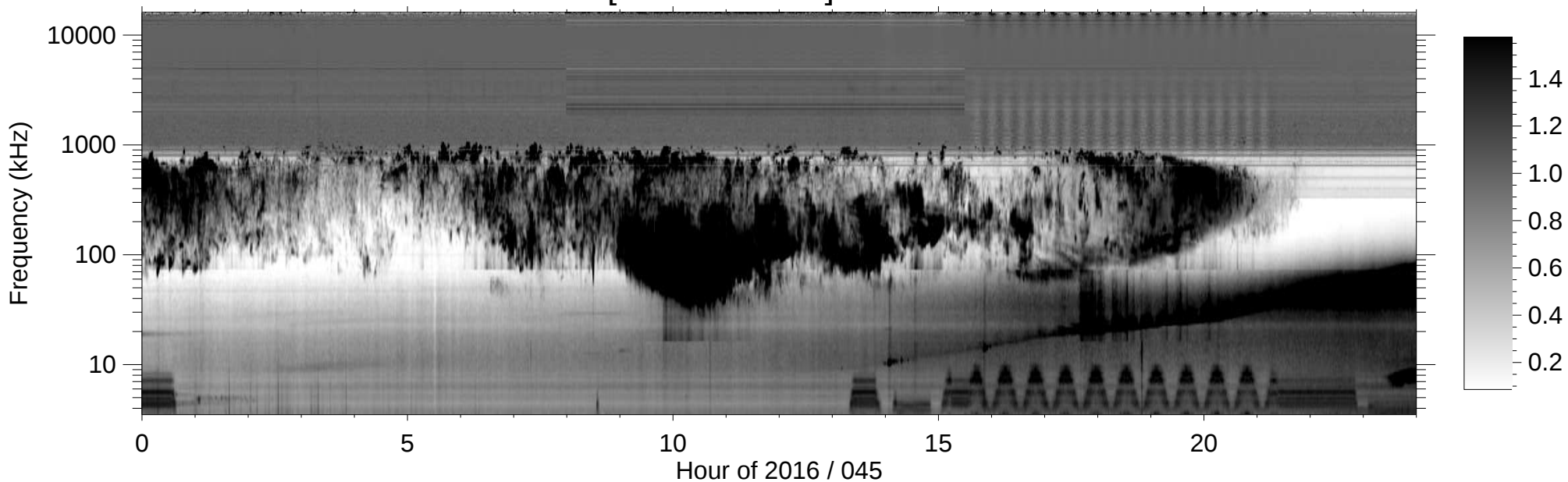
RPWS [ABCH1H2/Ex] (-B) 2016/02/14
