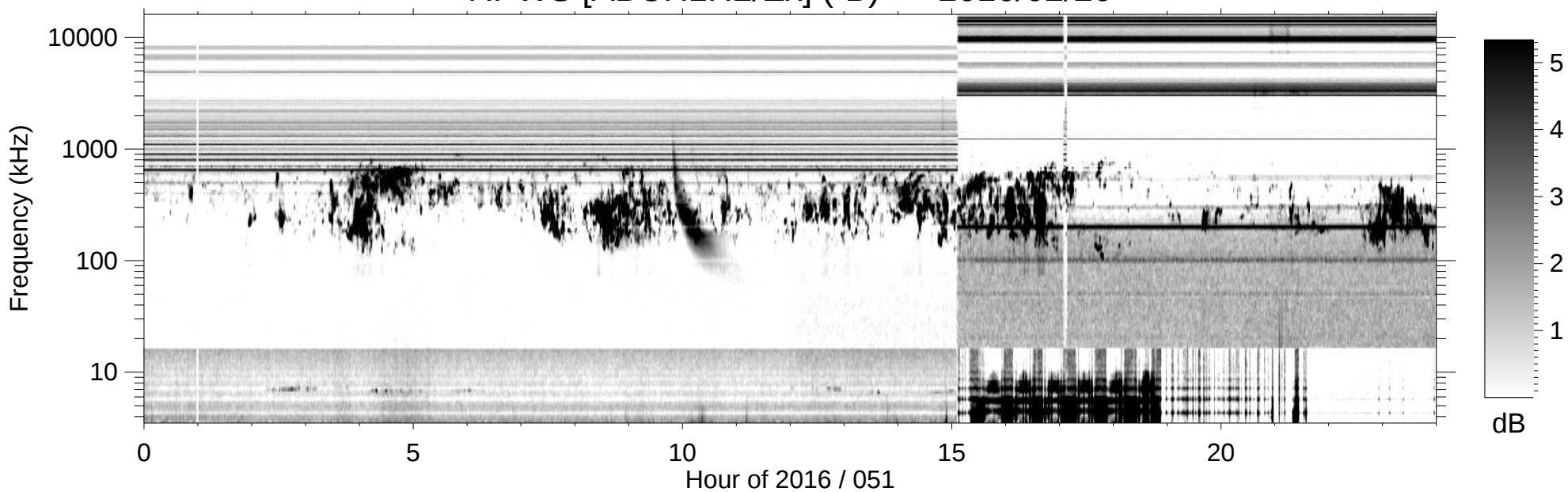
RPWS [ABCH1H2/Ex] (-B) 2016/02/20
