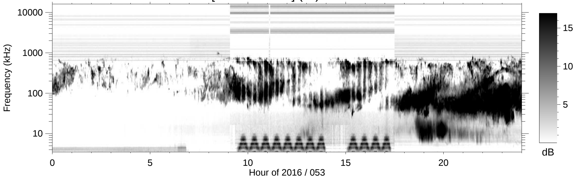
RPWS [ABCH1H2/Ex] (-B) 2016/02/22
