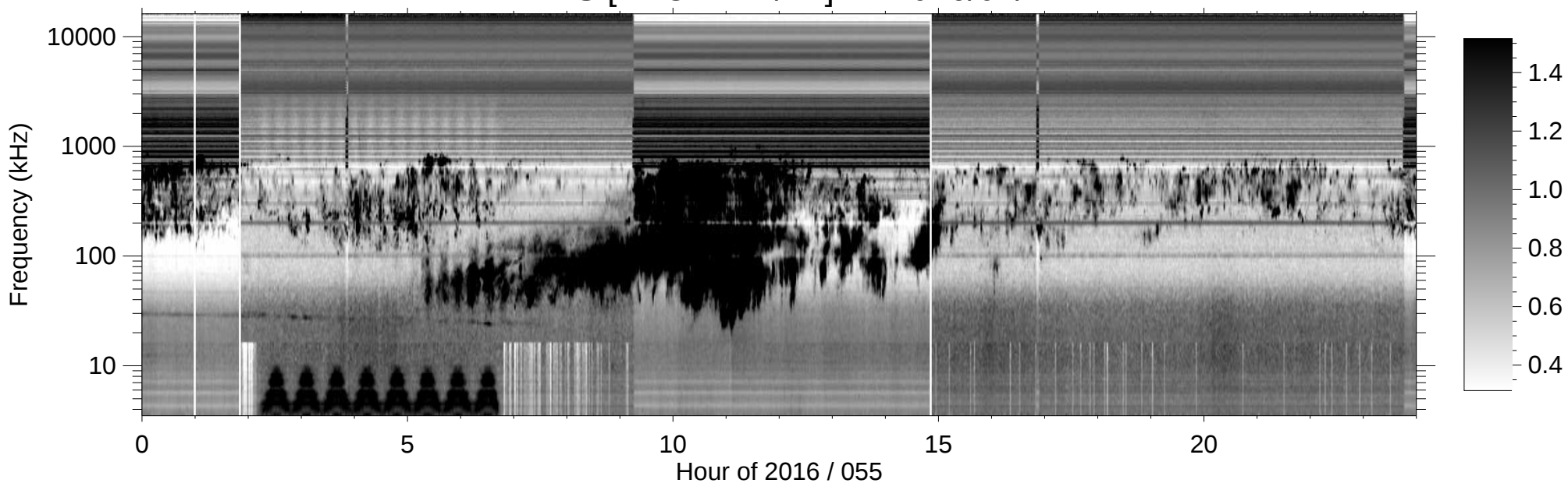
RPWS [ABCH1H2/Ex] (-B) 2016/02/24
