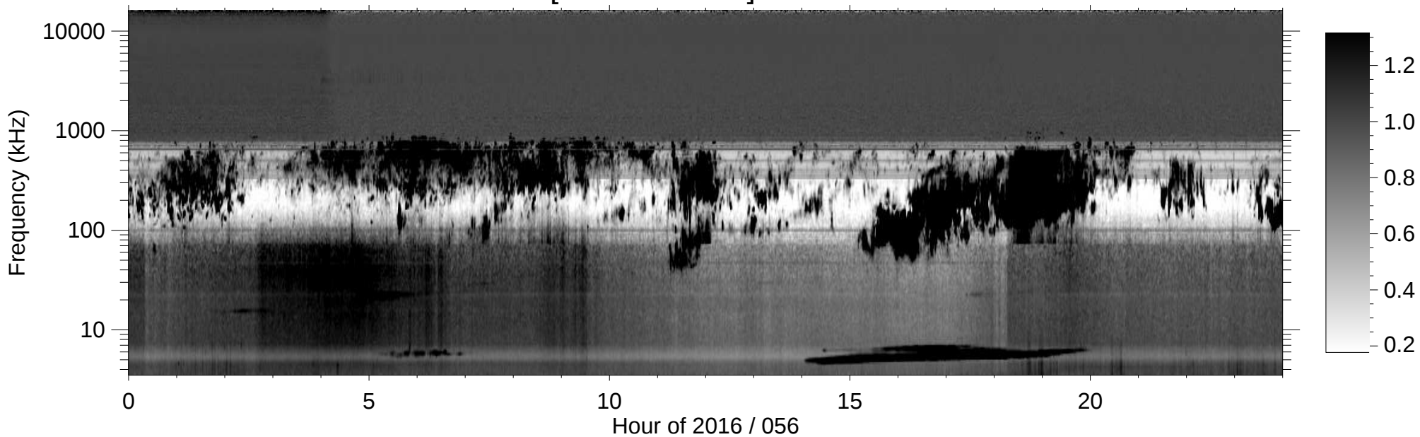
RPWS [ABCH1H2/Ex] (-B) 2016/02/25
