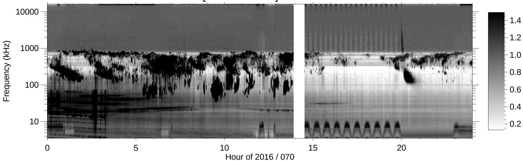
RPWS [ABCH1H2/Ex] (-B) 2016/03/10
