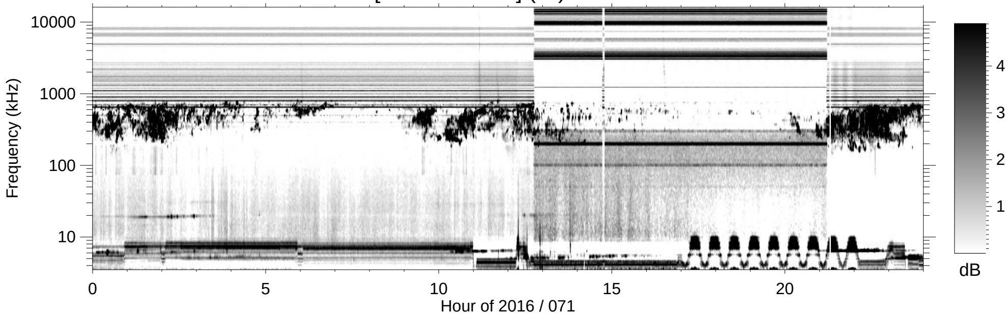
RPWS [ABCH1H2/Ex] (-B) 2016/03/11
