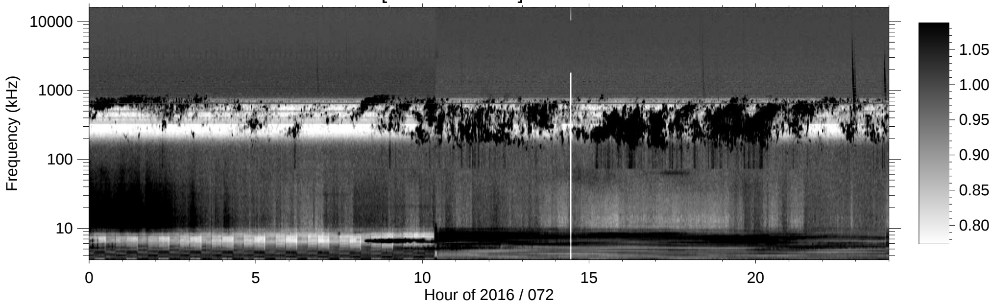
RPWS [ABCH1H2/Ex] (-B) 2016/03/12
