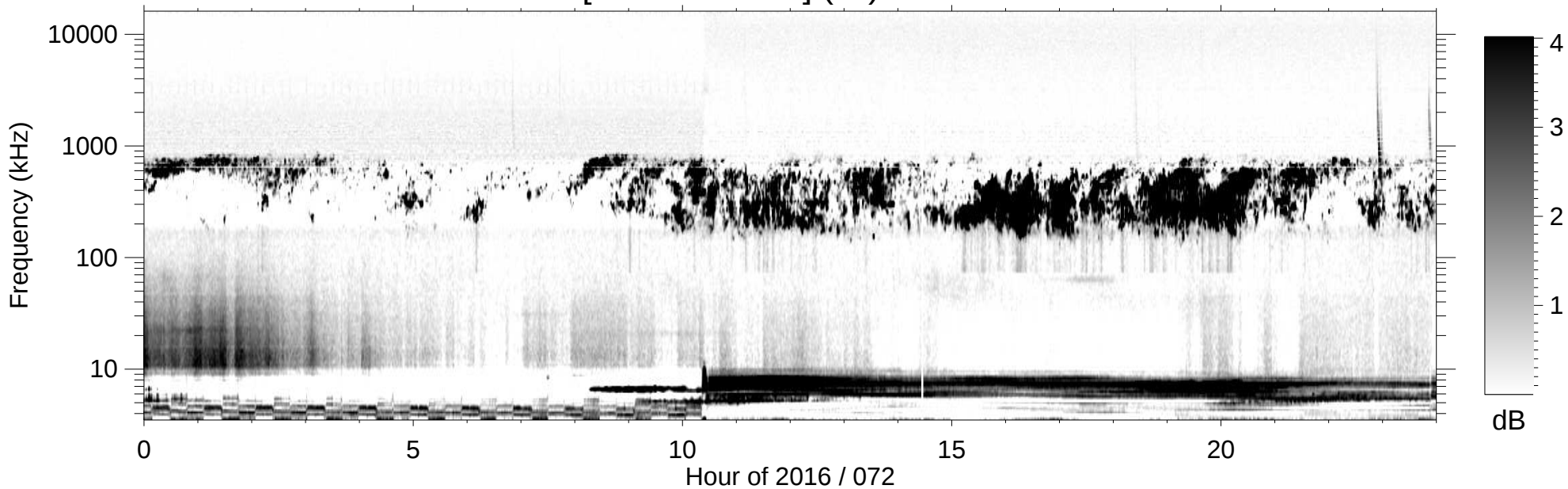
RPWS [ABCH1H2/Ex] (-B) 2016/03/12
