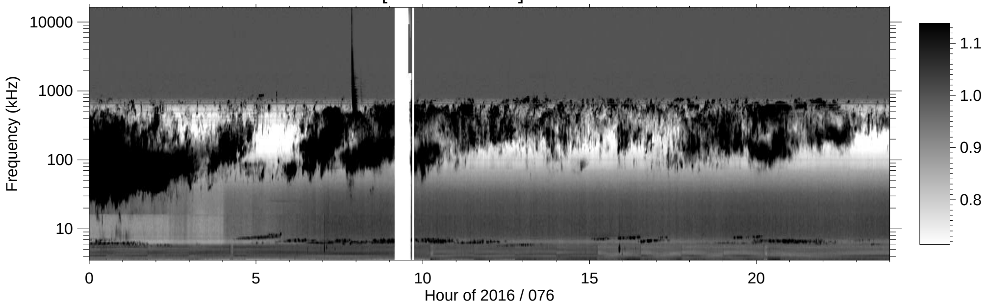
RPWS [ABCH1H2/Ex] (-B) 2016/03/16
