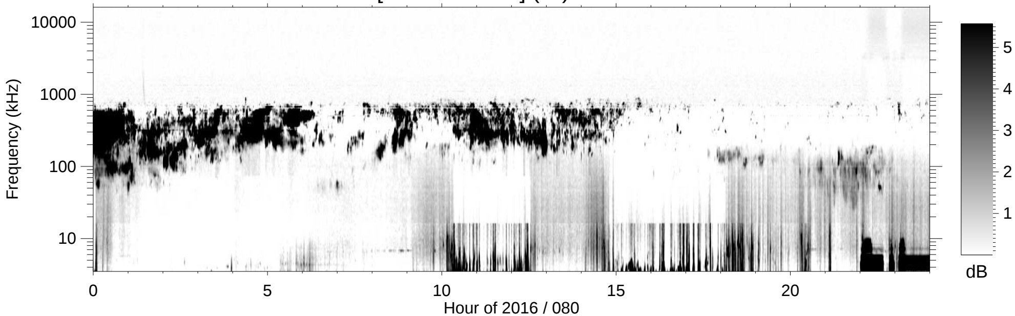
RPWS [ABCH1H2/Ex] (-B) 2016/03/20
