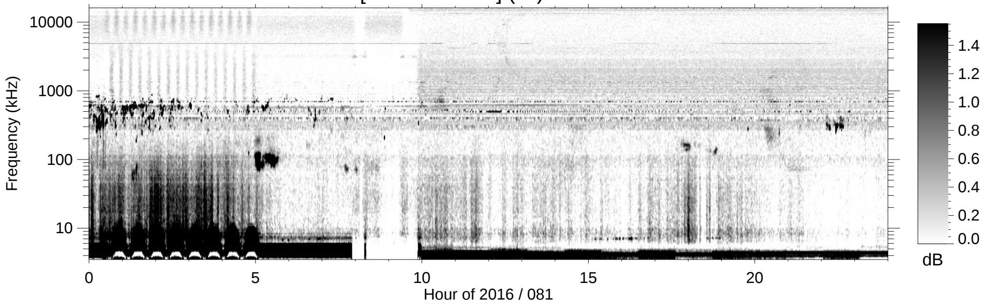
RPWS [ABCH1H2/Ex] (-B) 2016/03/21
