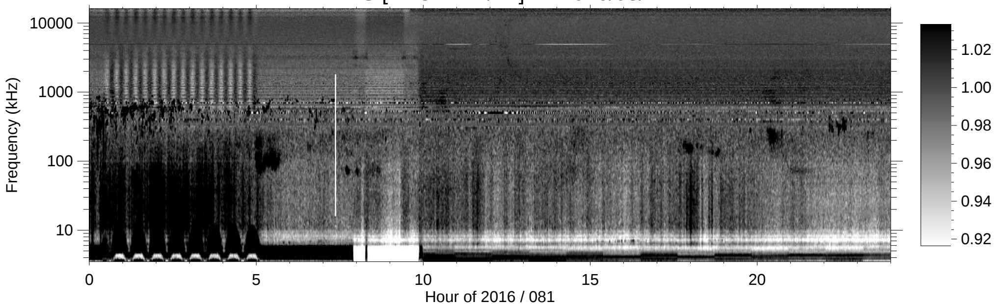
RPWS [ABCH1H2/Ex] (-B) 2016/03/21
