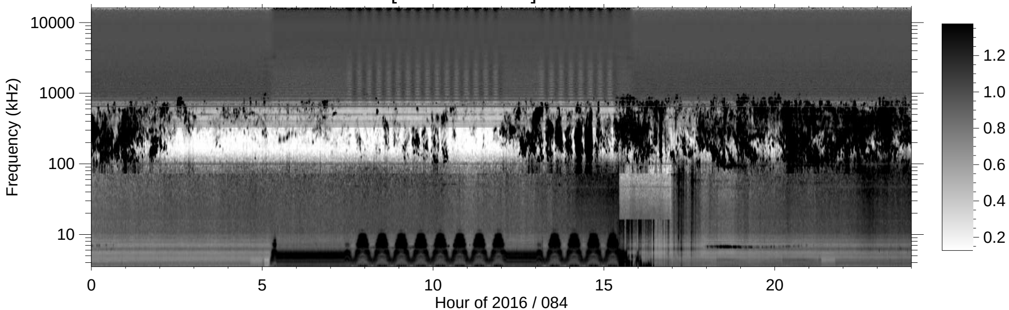
RPWS [ABCH1H2/Ex] (-B) 2016/03/24
