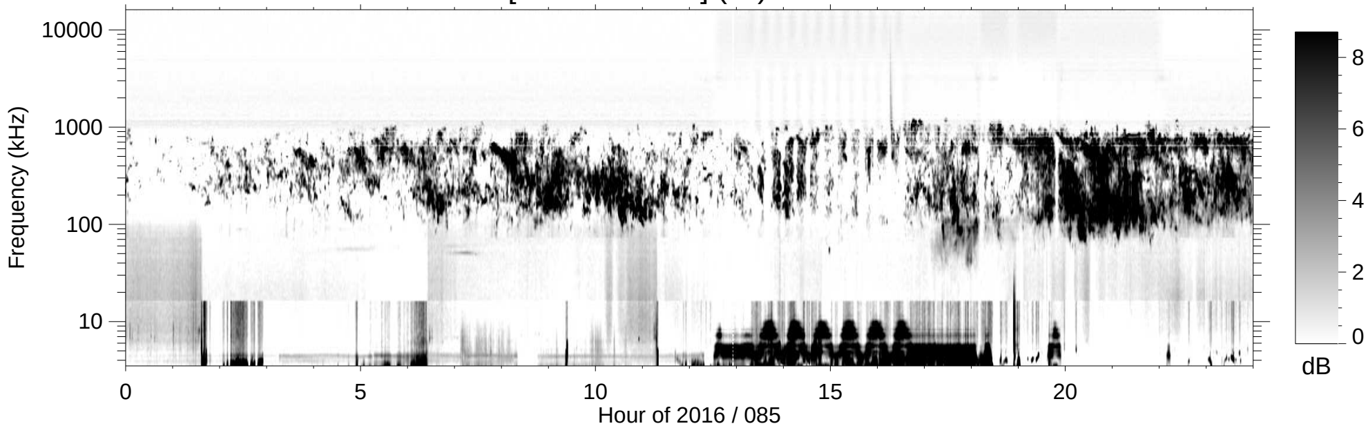
RPWS [ABCH1H2/Ex] (-B) 2016/03/25
