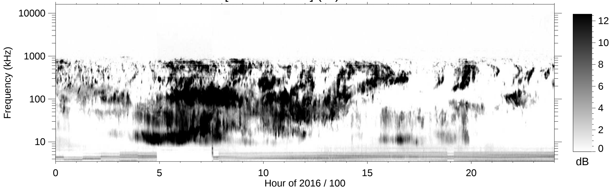
RPWS [ABCH1H2/Ex] (-B) 2016/04/09
