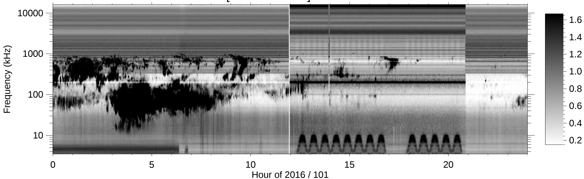
RPWS [ABCH1H2/Ex] (-B) 2016/04/10
