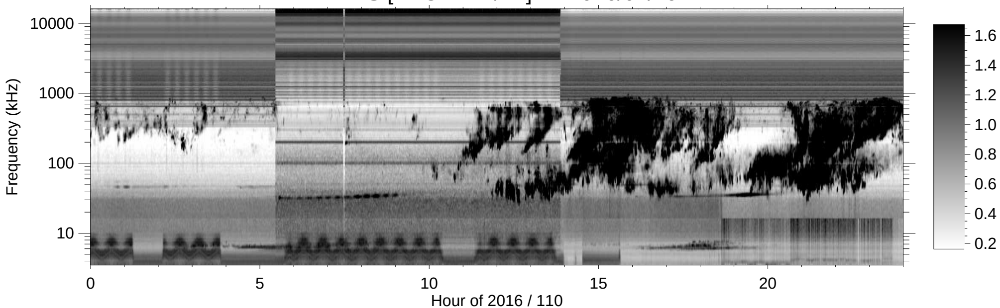
RPWS [ABCH1H2/Ex] (-B) 2016/04/19
