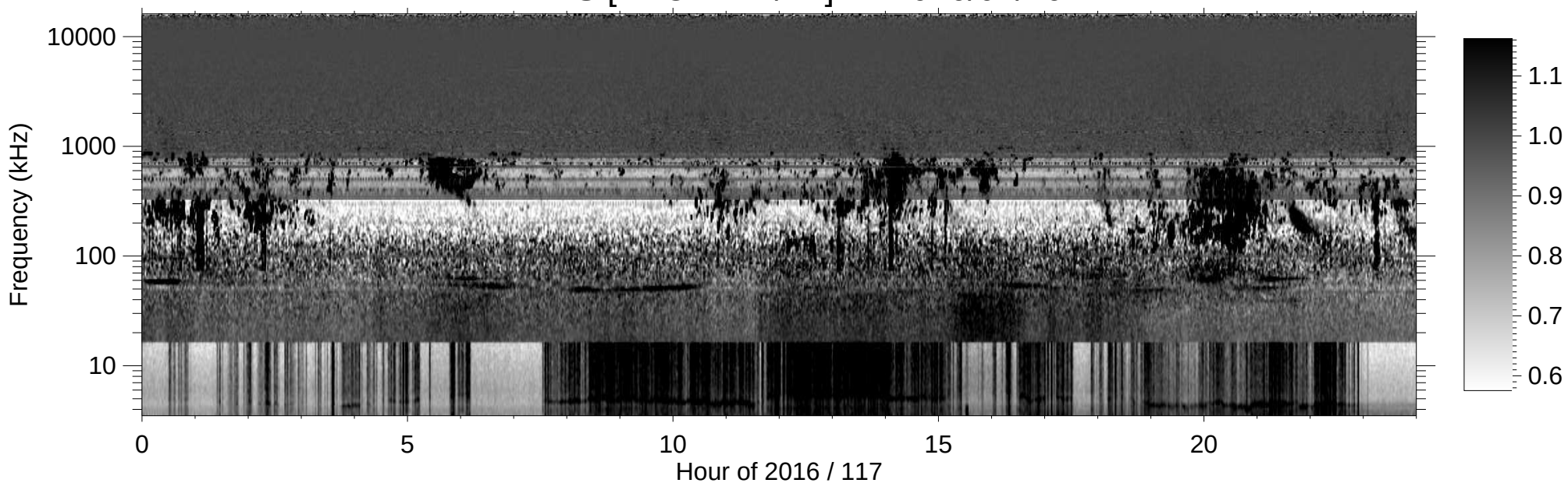
RPWS [ABCH1H2/Ex] (-B) 2016/04/26
