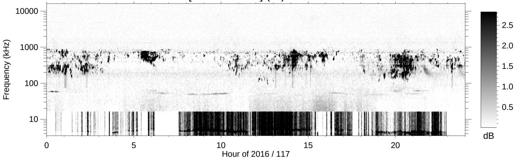
RPWS [ABCH1H2/Ex] (-B) 2016/04/26
