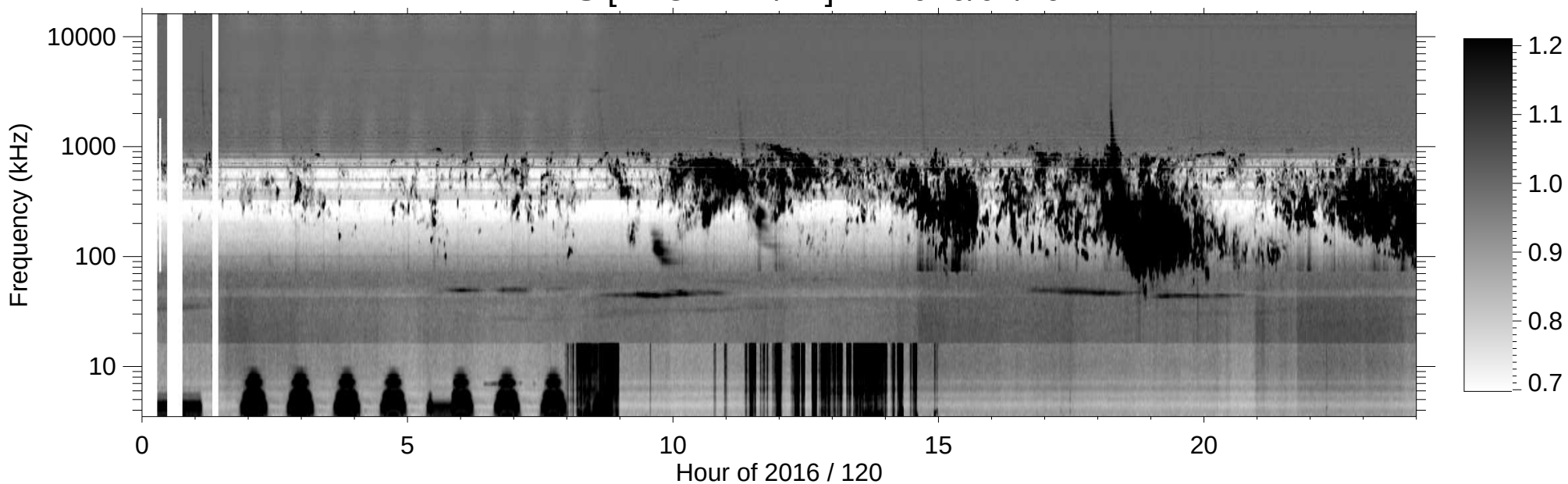
RPWS [ABCH1H2/Ex] (-B) 2016/04/29
