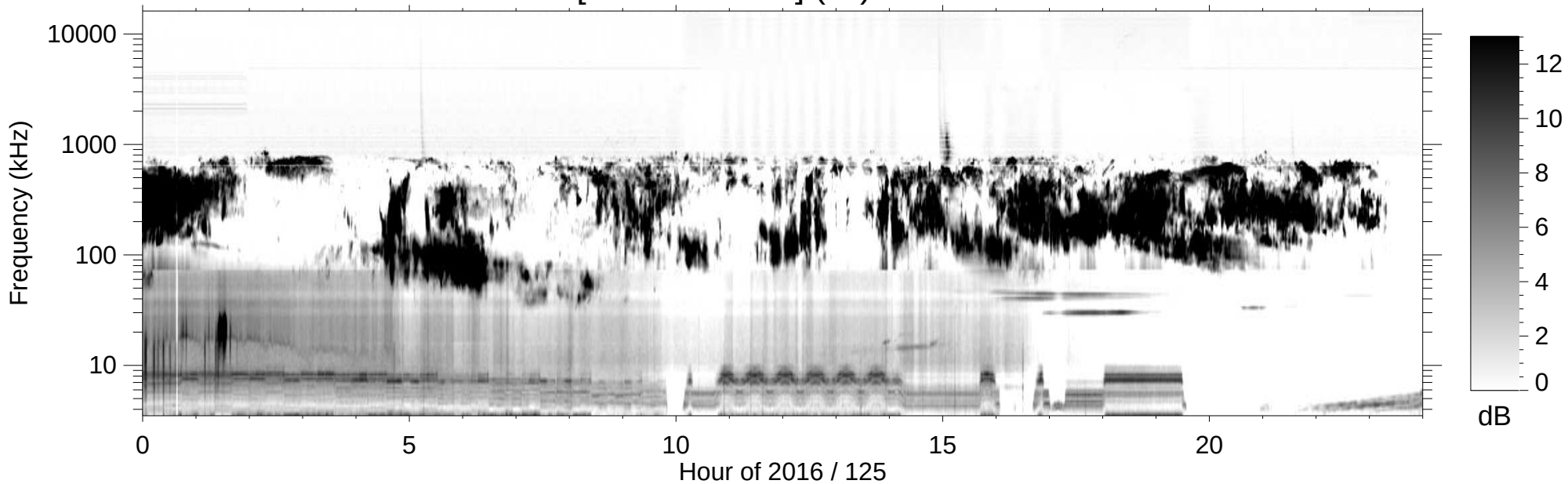
RPWS [ABCH1H2/Ex] (-B) 2016/05/04
