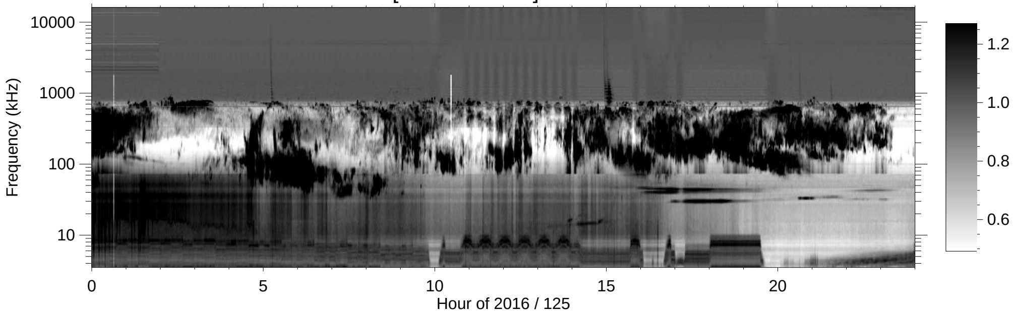
RPWS [ABCH1H2/Ex] (-B) 2016/05/04
