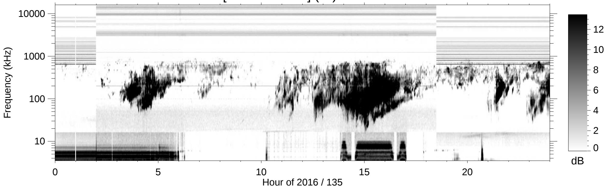
RPWS [ABCH1H2/Ex] (-B) 2016/05/14
