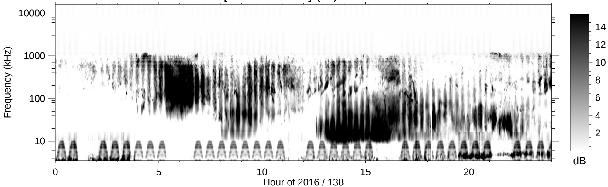
RPWS [ABCH1H2/Ex] (-B) 2016/05/17
