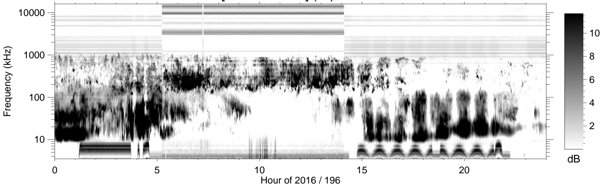
RPWS [ABCH1H2/Ex] (-B) 2016/07/14
