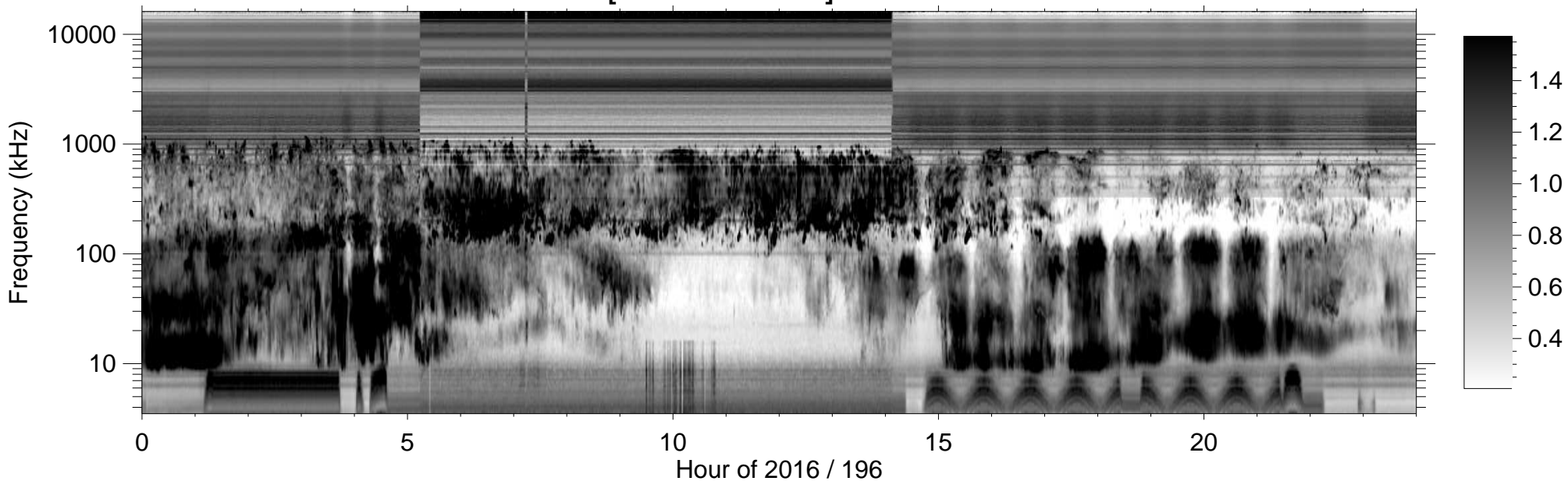
RPWS [ABCH1H2/Ex] (-B) 2016/07/14
