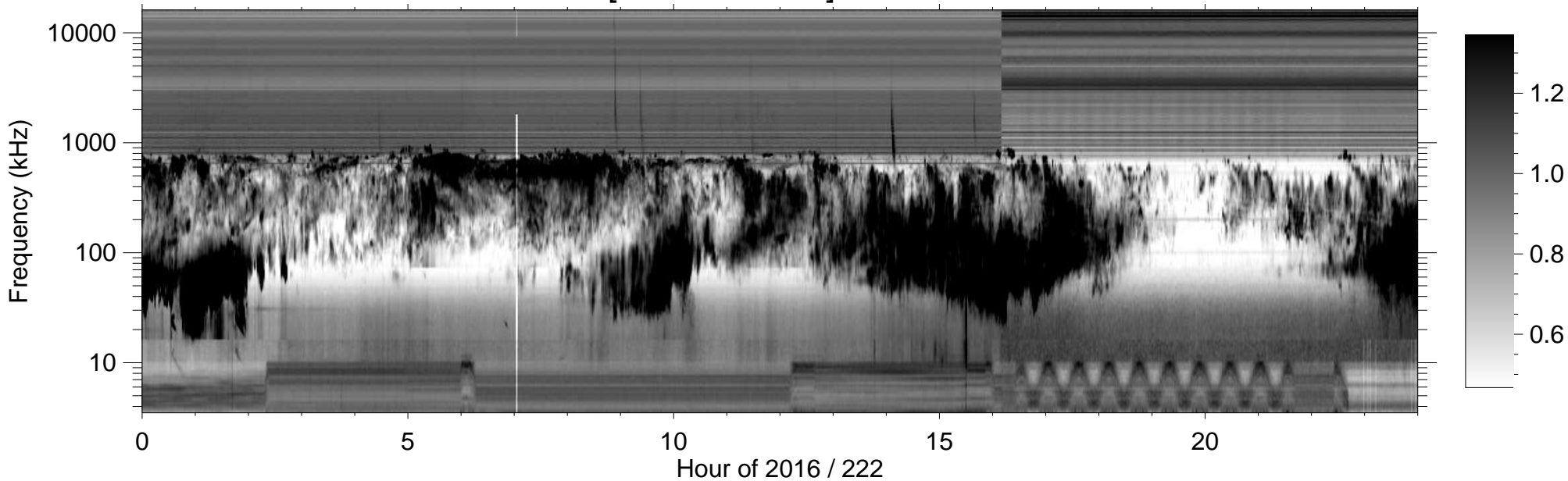
RPWS [ABCH1H2/Ex] (-B) 2016/08/09
