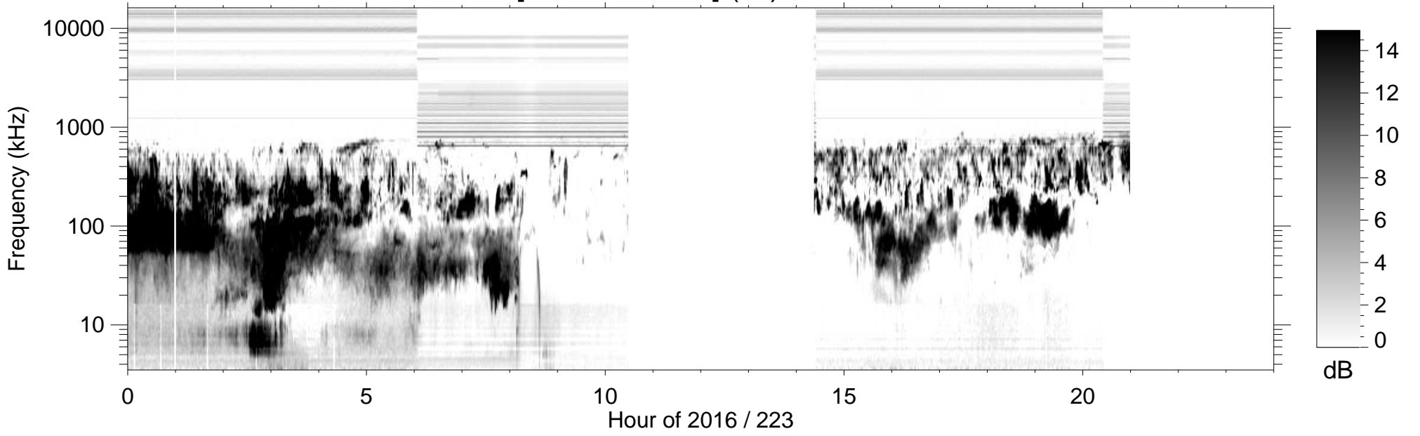
RPWS [ABCH1H2/Ex] (-B) 2016/08/10
