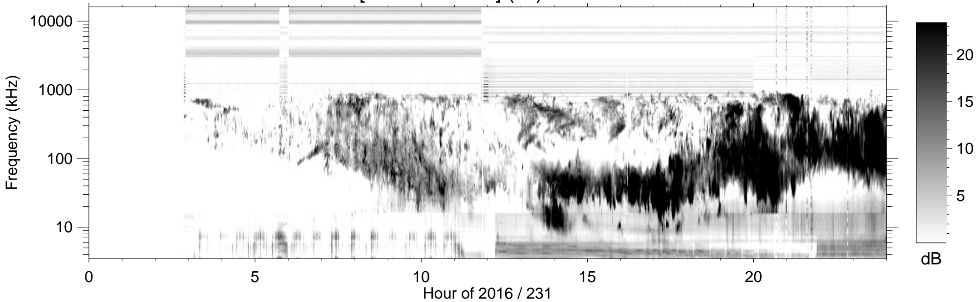
RPWS [ABCH1H2/Ex] (-B) 2016/08/18
