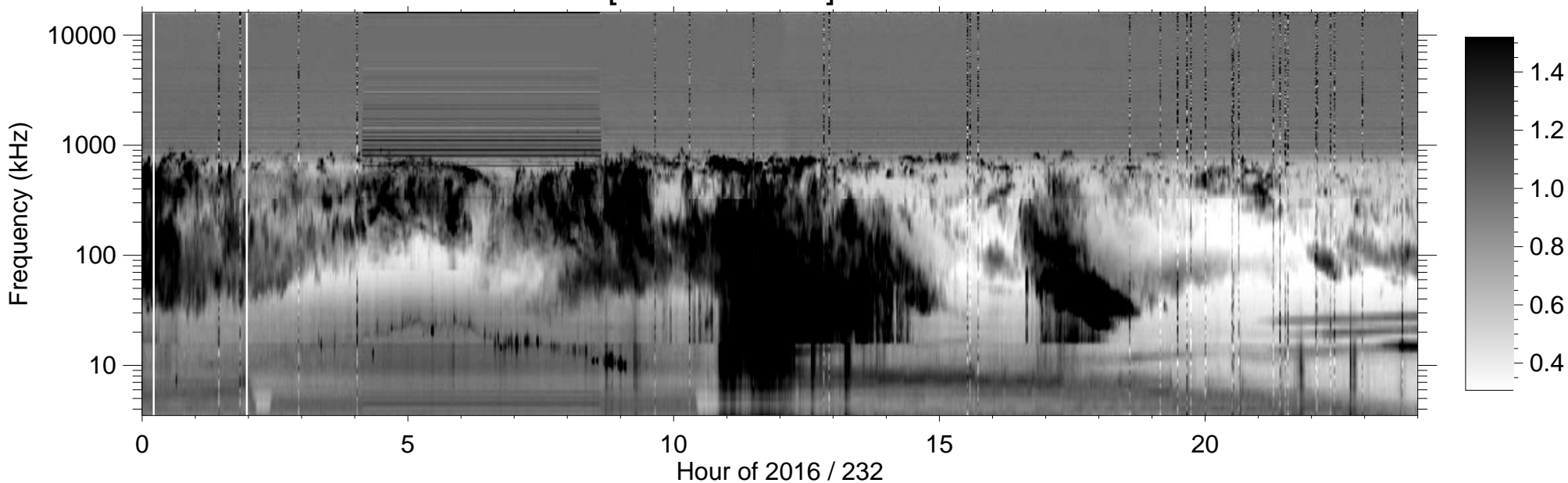
RPWS [ABCH1H2/Ex] (-B) 2016/08/19
