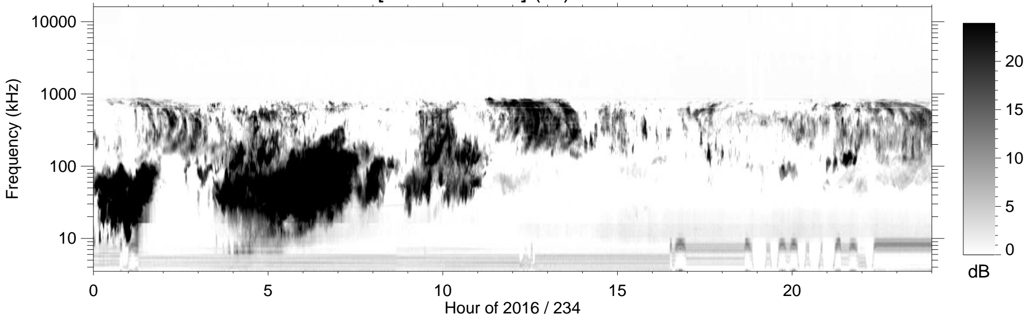
RPWS [ABCH1H2/Ex] (-B) 2016/08/21
