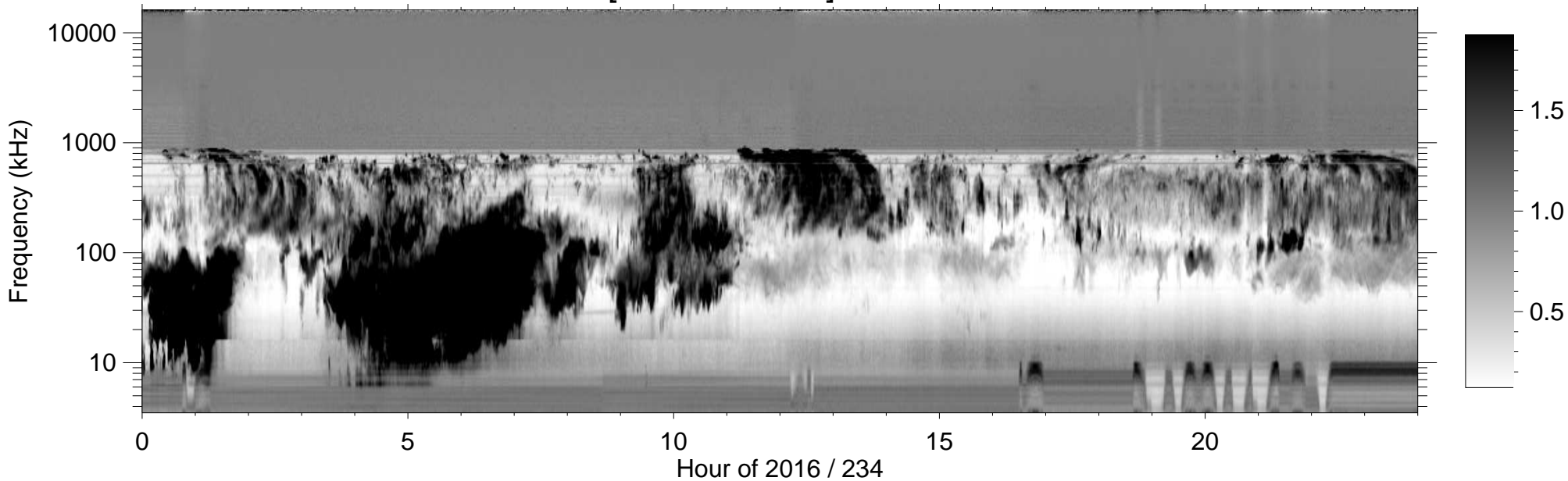
RPWS [ABCH1H2/Ex] (-B) 2016/08/21
